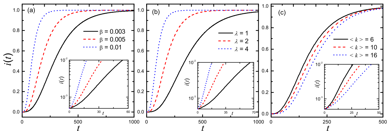
FIG. 1. Density of infected nodes i(t) as a function of time t for (a) different values of the spreading rate \beta , (b) different values of the packet-generation rate \lambda , and (c) different values of the average connectivity \langle k \rangle . For (a), \lambda = 2 and \langle k \rangle = 10 ; For (b), \beta = 0.005 and \langle k \rangle = 10 ; For (c), \beta = 0.005 and \lambda = 2 . The insets show the evolution of i(t) in the early times.
