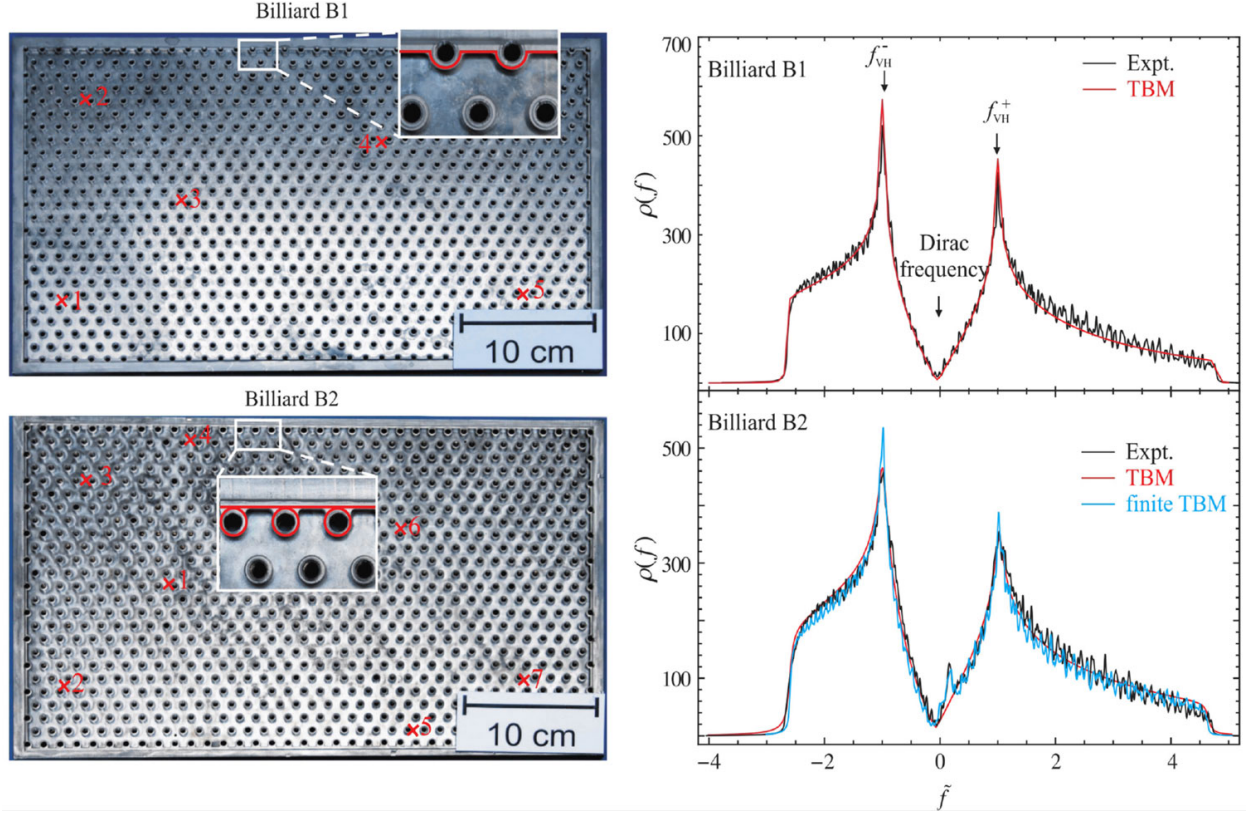
FIG. 3. Basin plates of microwave Dirac billiards and the corresponding density of states. Left: two billiards with different boundaries, each containing 888 metal cylinders. Right: the corresponding density of eigenfrequencies from experiments and from an infinite size tight-binding model. Lower panel: results from the tight-binding model of the same size as the experimental system. Modified from Ref. [224] with permission.
