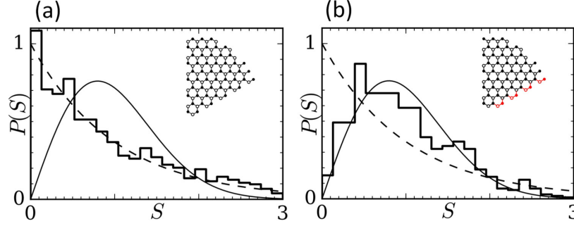
FIG. 21. Effect of structural perturbation on the nearest-neighbor spacing distribution for a graphene billiard with the shape of a 60^\circ sector. (a) armchair edges, (b) armchair edges with one row of atoms added along one edge. The energy range is E/t \in [0.02, 0.2] . Insets: magnified view of the lattice structure close to the tip of the sector to illustrate the differences. Adapted from Ref. [120] with permission.
