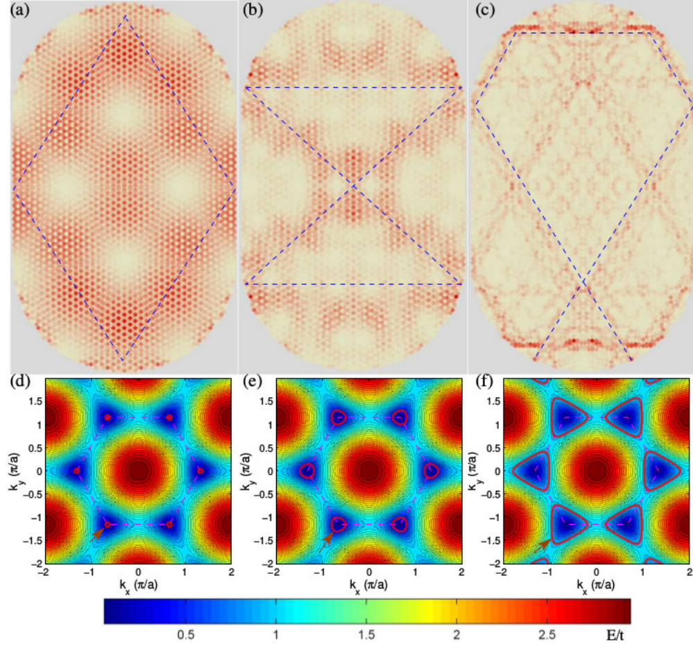
FIG. 23. Quantum scars in a chaotic graphene billiard of stadium geometry. Red color indicates higher wavefunction concentration associated with the scars. The stadium billiard contains N = 11814 carbon atoms and has zigzag horizontal boundaries. The energy contour plots in the wavevector plane (the band structure) are also shown. The energies for the patterns in (a-c) are E/t = 0.13252 , 0.4024 , and 0.91188 , respectively. Panels (d-f) show the E - \mathbf{k} configuration for an infinite graphene flake for the same lattice orientation and energy values as those for (a-c), respectively. The allowed wavevectors are on the constant energy curves (as indicated by the red arrows). Dashed line segments in (a-c) are for eye-guidance, and they indicate certain classical unstable periodic orbits. From Ref. [121] with permission.
