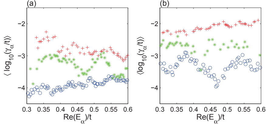
FIG. 43. Detailed behaviors of Fano resonance width for systems with different types of classical dynamics. Shown are the the mean values of \log_{10}(\gamma_\alpha/t) in a moving window with window size 0.04t and step size 0.004t . The upper curves in different panels in Fig. 42 are excluded in the average as they account for the smooth variation rather than the sharp conductance resonances. Panel (a) is for BGQD (left panels in Fig. 42) and panel (b) is for NRQD (right panels in Fig. 42). The blue circles, green asterisks, and red plus symbols are for mixed, intermediate, and chaotic dynamics in the classical limit, respectively. From Ref. [379] with permission.
