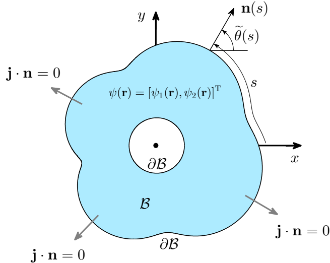
FIG. 69. Illustration of a paradigmatic system for studying persistent currents. Shown is a chaotic ring domain with boundary parameterized by the arc length s . For motion of a massless Dirac fermion inside the domain, the boundary condition is of the zero-flux type, i.e., no outward current at any point s : \mathbf{j} \cdot \mathbf{n} = 0 . From Ref. [137] with permission.
