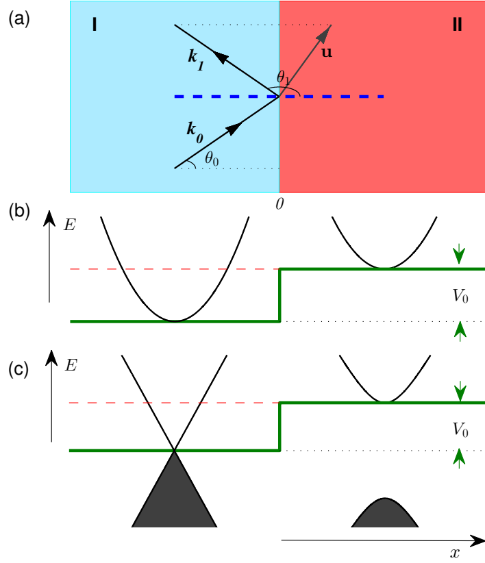
FIG. 73. Setting of analytic model to understand SPCs. Shown are incident, reflected and transmitted local plane waves at a potential jump. From Ref. [137] with permission.
