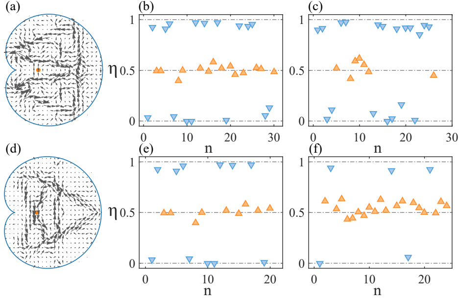
FIG. 31. Directions of currents associated with period-5 scars in the AB chaotic Dirac billiard. The same plots as in Fig. 29 except that the first and second rows are for the period-5-I and period-5-II scars listed in Tab. III, respectively. From Ref. [124] with permission.
