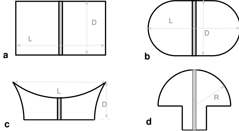
FIG. 60. Schematic illustration of four classes of geometrical domains for graphene billiards used to study the interplay among chaos, relativistic quantum mechanics, and many-body effect: (a) rectangle, (b) stadium, (c) bowtie, and (d) mushroom. The respective classical dynamics are integrable (a), chaotic with neutral periodic orbits (b), hyperbolic with all periodic orbits being unstable (c), and nonhyperbolic with a mixed phase space (d). The thin gray region along a symmetric line represents the potential barrier.
