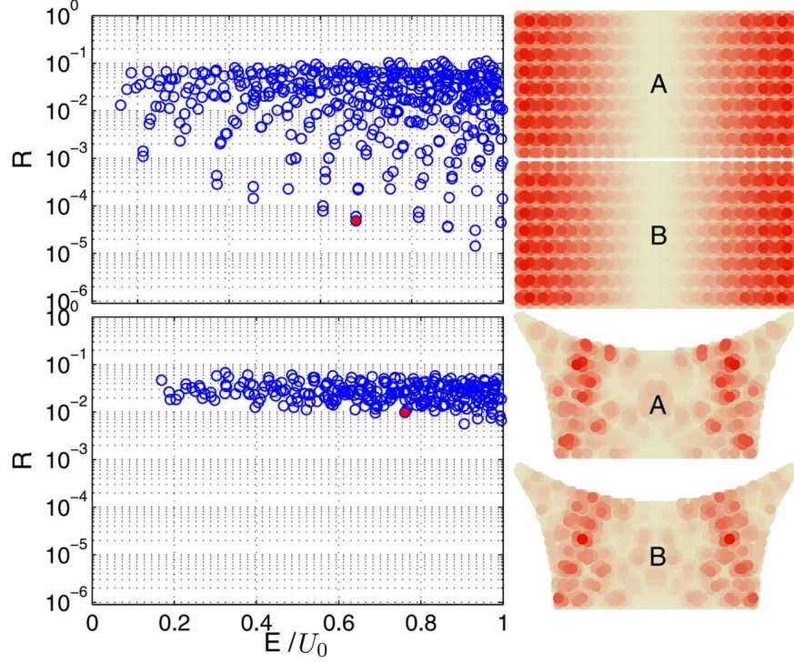
FIG. 51. Tunneling rates and LDS patterns in integrable and fully chaotic graphene double-well systems. For graphene, there are two distinct types of atoms in a unit cell, denoted as A and B . The tight-binding model was used to calculate the eigenstates. The barrier height is fixed at U_0 \sim 0.67t . After converting to the \hbar = c = 1 unit system, the geometric measures and the barrier potential are the same as those for Fig. 50. From Ref. [134] with permission.
