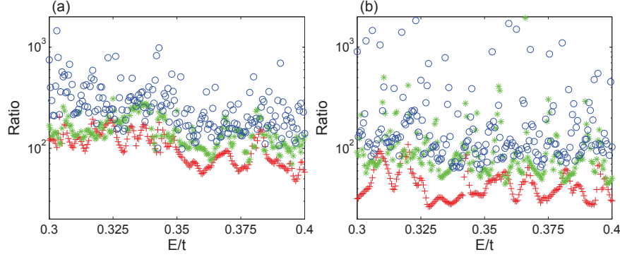
FIG. 45. Characterization of the degree of localization of quantum states for BGQDs. Shown are the values of the ratio of the maximum to the minimum values of the LDS versus energy: (a) BGQD and (b) NRQD. From top to bottom the blue circles, green asterisks, and red plus symbols are for mixed, intermediate, and chaotic cases, respectively. From Ref. [379] with permission.
