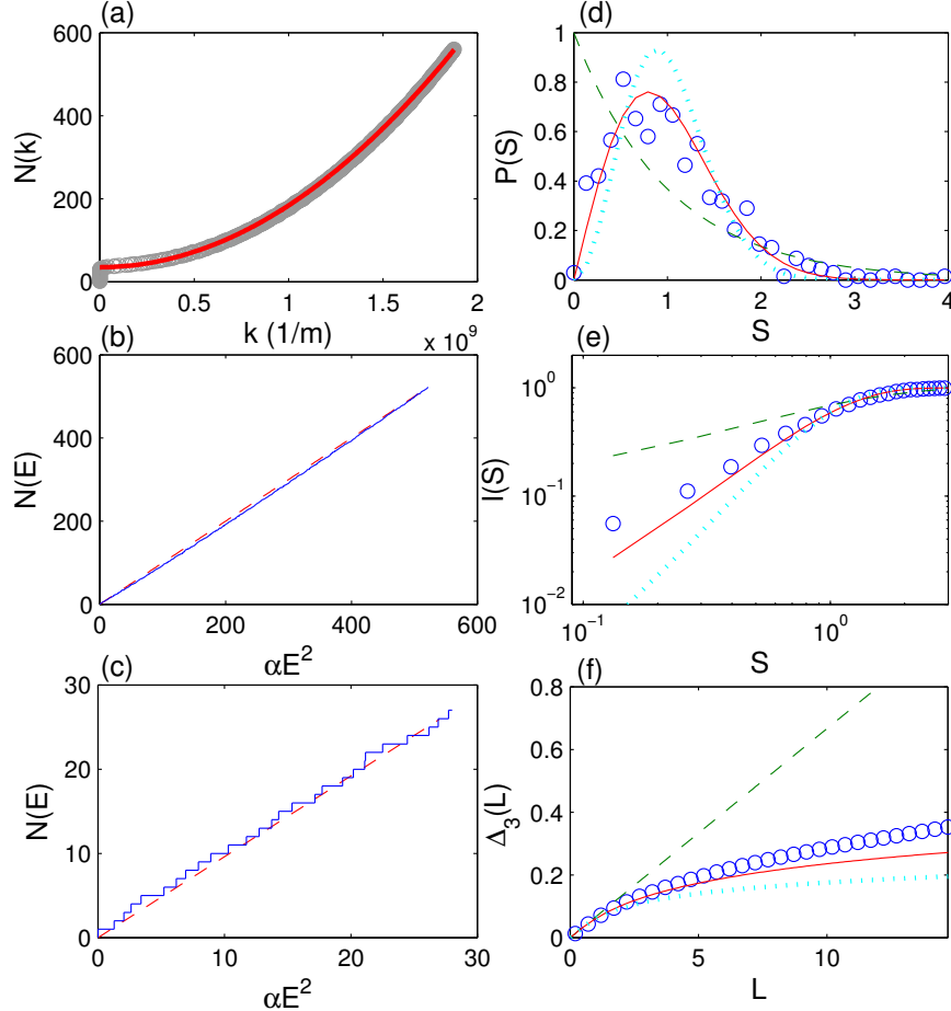
FIG. 15. Level-spacing statistics for the Africa shaped graphene billiard without any magnetic field ( \Phi = 0 ). (a) Wavevector staircase function N(k) for eigenenergies in the range 0 < E_n/t < 0.4 , where the number of energy levels is 560 (circles). The curve is given by \langle N(k) \rangle = Ak^2/(2\pi) + 35 [Eq. (118)]. (b) Spectral staircase function N(E) versus \alpha E^2 for 0.02 < E_n/t < 0.4 with 522 levels, where \alpha is the unfolding normalization constant. The dashed straight line is the averaged staircase function Eq. (119). (c) Magnification of part of (b) for 0.02 < E_n/t < 0.1 with 28 levels. (d) Unfolded level-spacing distribution P(S) . (e) Cumulative unfolded level-spacing distribution I(S) . (f) Spectral rigidity \Delta_3 . In (d-f), the numerical data are represented by open circles and the lines are theoretical predictions from the random matrix theory: dashed line for Poisson, solid line for GOE, and dotted line for GUE statistics. From Ref. [118] with permission.
