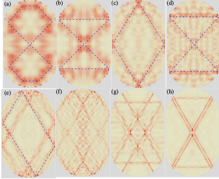
FIG. 24. Typical scars in the chaotic stadium graphene billiard with zigzag straight boundaries. A number of quantum scars for the same system as in Fig. 23. The energy values for (a-h) are E/t = 0.25347, 0.36358, 0.57665, 0.60699, 0.81956, 0.91061, 0.97722, \text{ and } 0.99198 , respectively. The dashed lines represent the corresponding classical periodic orbits. From Ref. [121] with permission.
