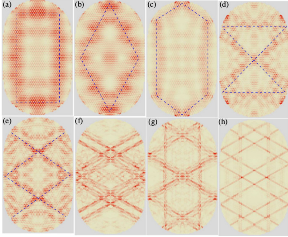
FIG. 25. Quantum scars in a chaotic stadium graphene billiard with armchair straight boundaries. The billiard has N = 13694 carbon atoms. The corresponding energy values are E/t = 0.20031, 0.2599, 0.3106, 0.54954, 0.59238, 0.9168, 0.95216, \text{ and } 0.99801 for (a-h), respectively. From Ref. [121] with permission.
