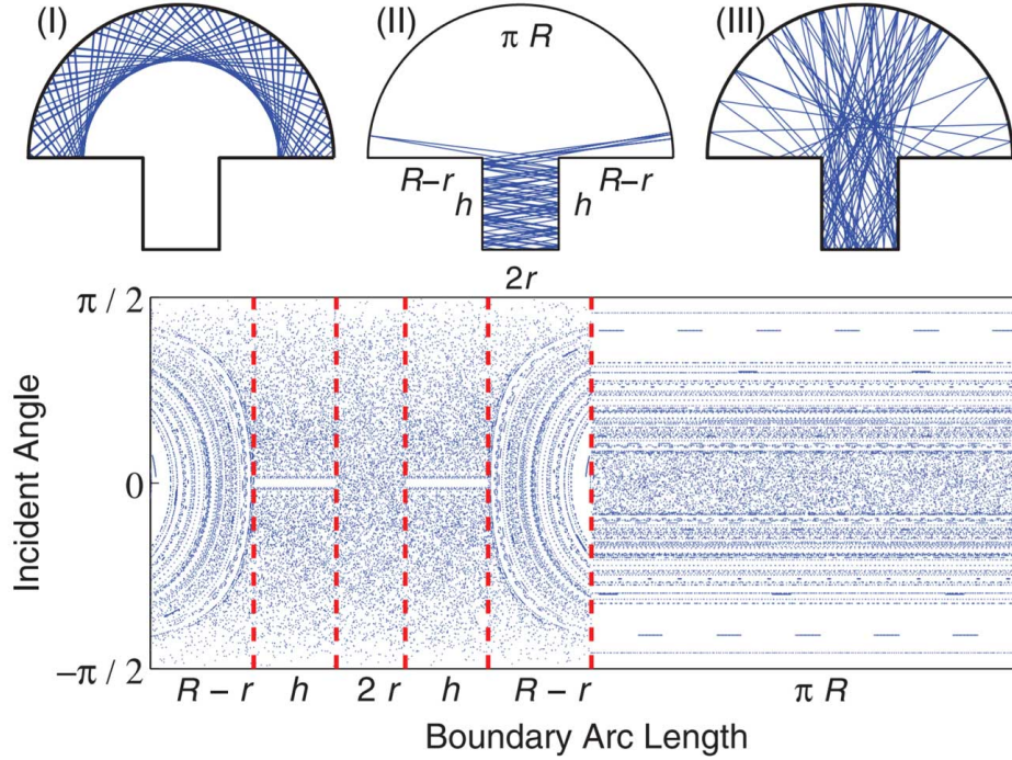
FIG. 52. Nonhyperbolic classical dynamics of the mushroom billiard. The mushroom billiard consists of a semicircular cap and a rectangular stem. The top row show three different types (I, II, III) of classical trajectories: stable, marginally stable periodic, and chaotic orbits. The bottom panel depicts the discrete time map in the phase space defined by the boundary arc length and the incident angle. The regions separated by the red vertical dashed lines correspond to the line/arc boundary segments marked in (II). From Ref. [135] with permission.
