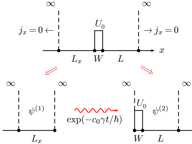
FIG. 56. One-dimensional “toy” resonant tunneling model. Schematic diagram for one-dimension tunneling of a massless Dirac fermion.
