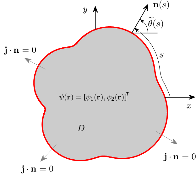
FIG. 4. Illustration of a 2D Dirac billiard domain and the boundary conditions. The domain boundary is parametrized by arc length s . For motion of a massless Dirac fermion inside the domain, the boundary conditions are of the zero-flux type, i.e., no outward current at any point s : \mathbf{j} \cdot \mathbf{n} = 0 , which is equivalent to \psi_2/\psi_1 = i \exp[i\tilde{\theta}(s)] with \tilde{\theta}(s) being the argument of the outward normal \mathbf{n}(s) .
