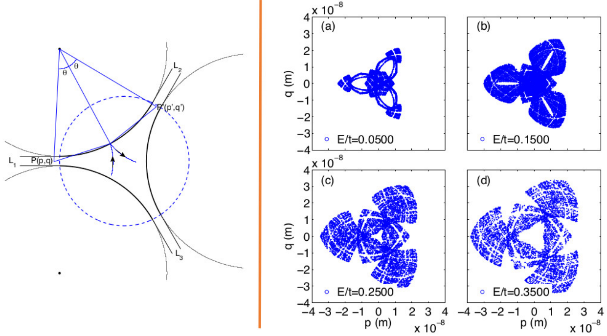
FIG. 46. An illustrative three-terminal classical chaotic scattering system in the presence of a magnetic field, whose dynamical invariant set depends on the electron Fermi energy. Left half: geometry of a three-terminal quantum dot system. The boundary of the device is indicated by the black heavy lines. A perpendicular magnetic field is applied in the circular region defined by the blue dashed lines. The system is made entirely of graphene. The corresponding classical dynamics is effectively that of an open billiard system with three outgoing channels. Right half: for a fixed magnetic field specified by \Phi/\Phi_0 = 0.0019 , representative chaotic sets for four different values of the Fermi energy: (a) E/t = 0.05 , (b) E/t = 0.15 , (c) E/t = 0.25 , and (d) E/t = 0.35 , where p and q are the coordinates of center points of the electron trajectory. It can be seen that the chaotic sets are characteristically distinct.
