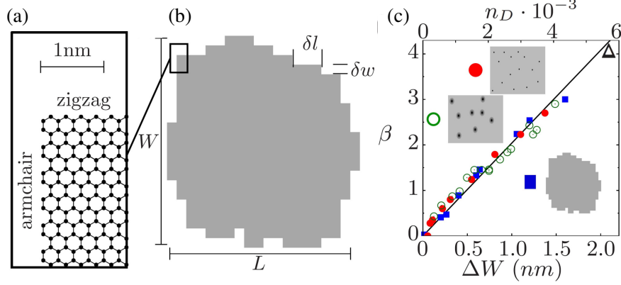
FIG. 13. Level spacing statistics of a graphene flake in the absence or presence of random disorders.
