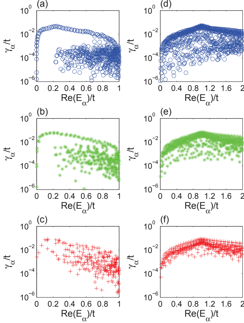
FIG. 42. Characteristics of Fano resonances in BGQDs. Shown are the resonance width \gamma_\alpha for bi-layer graphene quantum dots and their nonrelativistic quantum counterparts for different types of classical dynamics: (a) BGQD/mixed (b) BGQD/intermediate (c) BGQD/chaotic, (d) NRQD/mixed (e) NRQD/intermediate, and (f) NRQD/chaotic. The energy values at which the self-energy is evaluated are E_0 = 0.2t for (a-c) and E_0 = t for (d-f). From Ref. [379] with permission.
