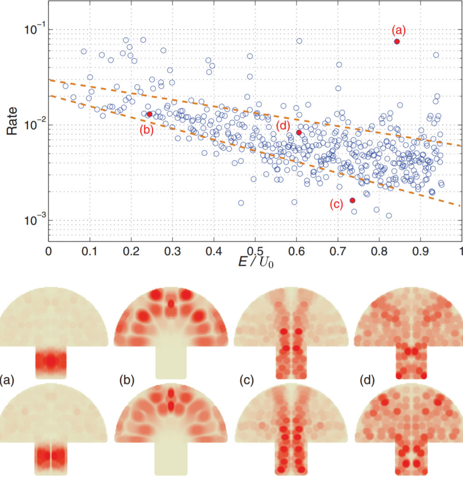
FIG. 53. Typical behaviors of tunneling rates and eigenstates for a massless Dirac fermion in the mushroom billiard. The billiard parameters are r = 0.25R and h = 0.6R . The height and width of the potential barrier are U_0 = 60 and w = 0.15 , respectively. The first and second rows of patterns show the intensity distributions of the \phi and \chi components of the Dirac spinor, respectively. The four red points in the tunneling-rate plot (upper panel) correspond to the patterns for (a) a marginally stable periodic orbit of type-II, (b) a stable periodic orbit of type-I, (c) an orbit with extremely low tunneling rate, and (d) a chaotic orbit of type-III. From Ref. [135] with permission.
